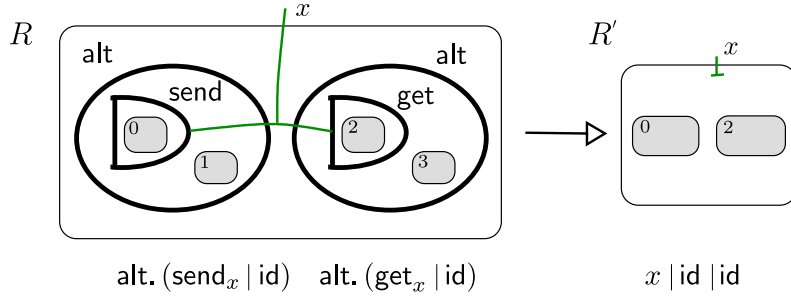
Fig. 8. The reaction rule (R, R', \eta) for \text{BIG}_{\text{CCS}} .
